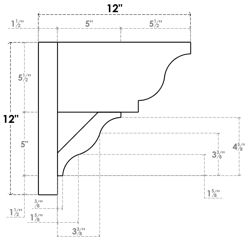
SIDE PROFILE
